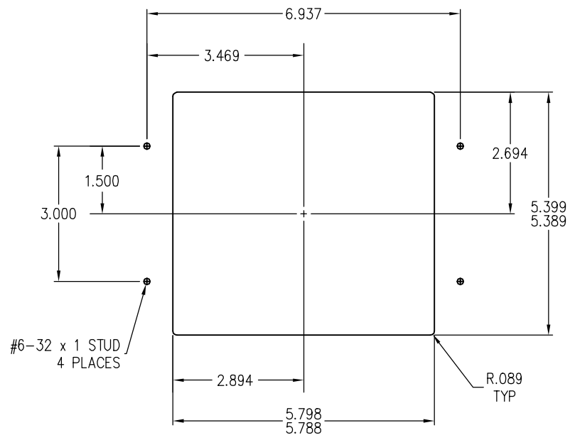
4x4 KEYPAD CUT OUT AND STUD DETAIL
