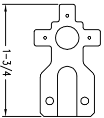
OPTIONAL END EFFECTOR KIT PART # RK-ID0043
